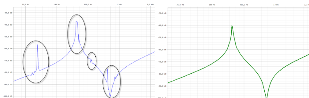
Figure 13: Capacitive interwinding on HV winding performed with SFRA Instrument 1 (left) and SFRA Instrument 2 (right)
