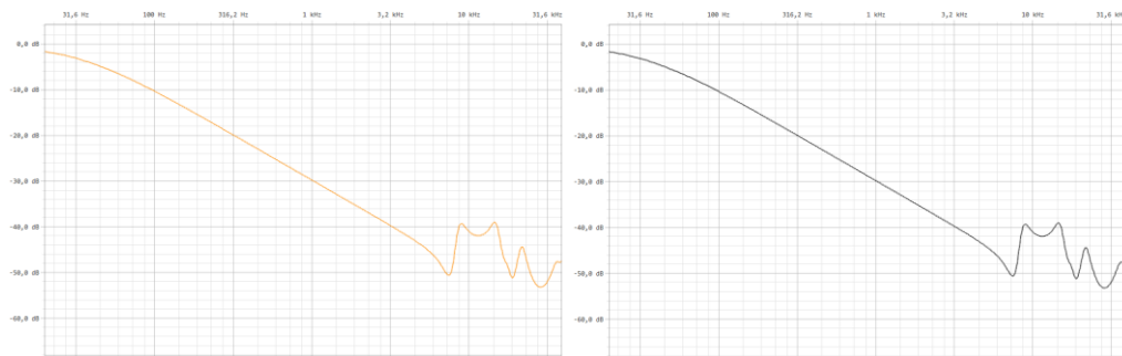
Figure 14: End-to-end short-circuit on HV winding performed with SFRA Instrument 1 (left) and SFRA Instrument 2 (right)
