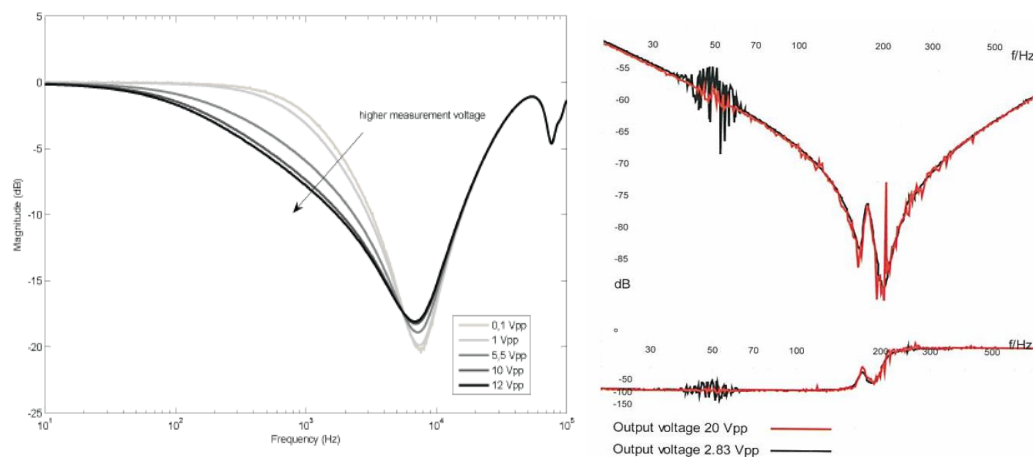
Figure 10: Effect of the selected output voltages left: influence of different output voltages on magnetization inductance L_m right: influence on narrowband noise suppression capabilities by using different output voltages
