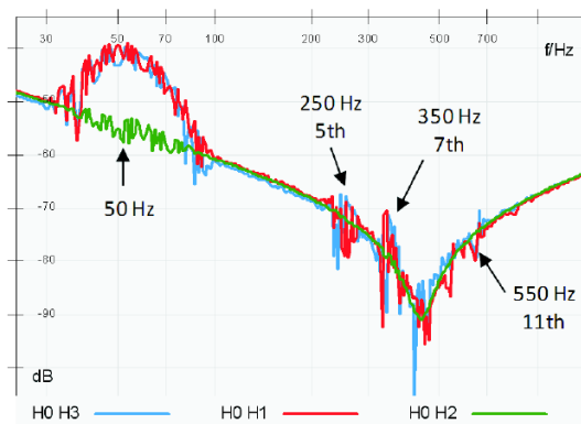
Figure 3: Sweep Frequency Response of a 500 kV Winding, with narrowband noise at power frequency and its harmonics
