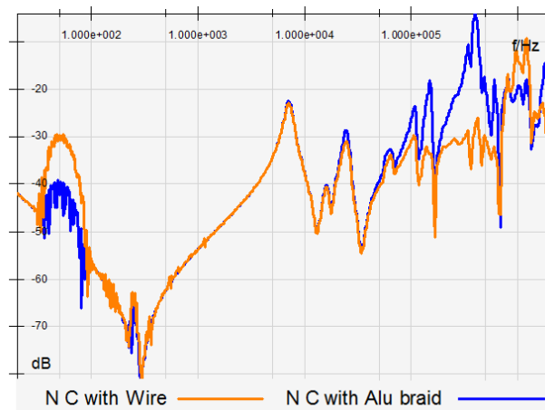
Figure 8: Effect of two different connection techniques, using a banana cable (4mm) and aluminium braid
