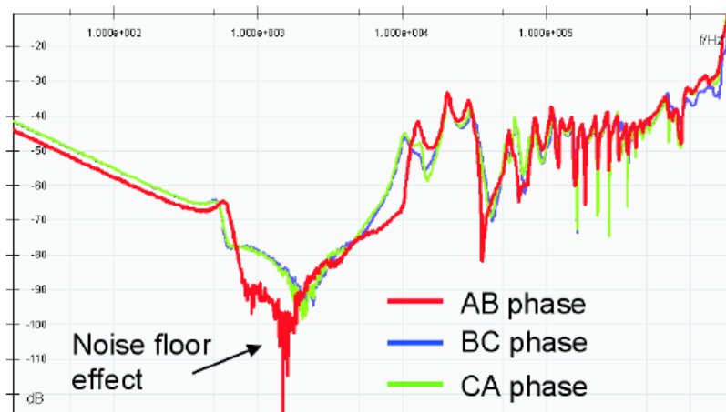
Figure 5: Example of the effect of noise floor in SFRA measurements in delta connected windings
