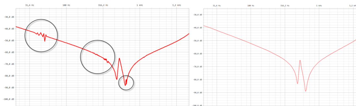
Figure 12: End-to-end open-circuit on HV winding performed with SFRA Instrument 1 (left) and SFRA Instrument 2 (right)
