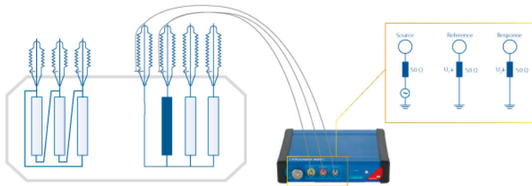
Figure 1 Typical setup of a transfer function measurement in frequency domain
