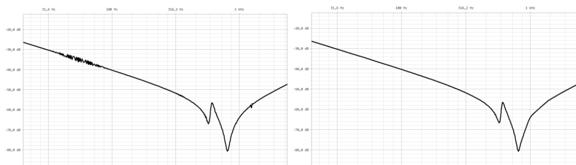
Figure 11: Comparison of the SFRA trace before (left) and after noise removal (right)
