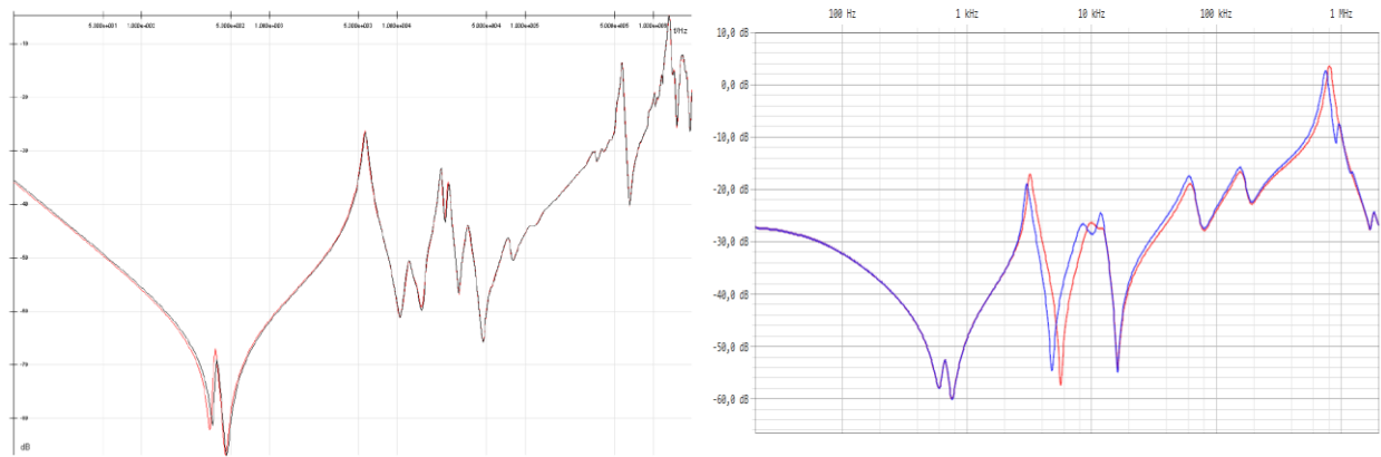
Figure 2 Typical frequency responses of power transformers left: healthy transformer, actual trace nearly identical to reference right: Bulk movement, actual trace shows significant deviations to reference
